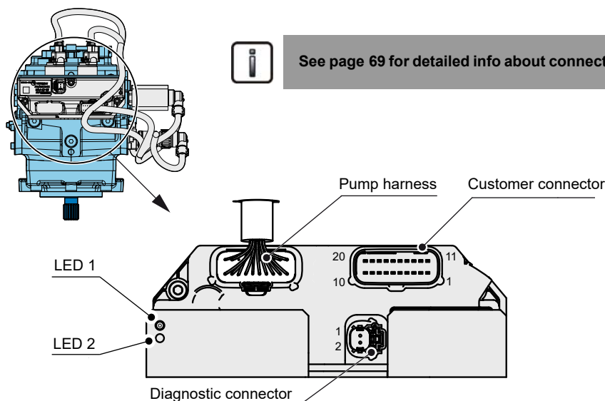
Customer connector
