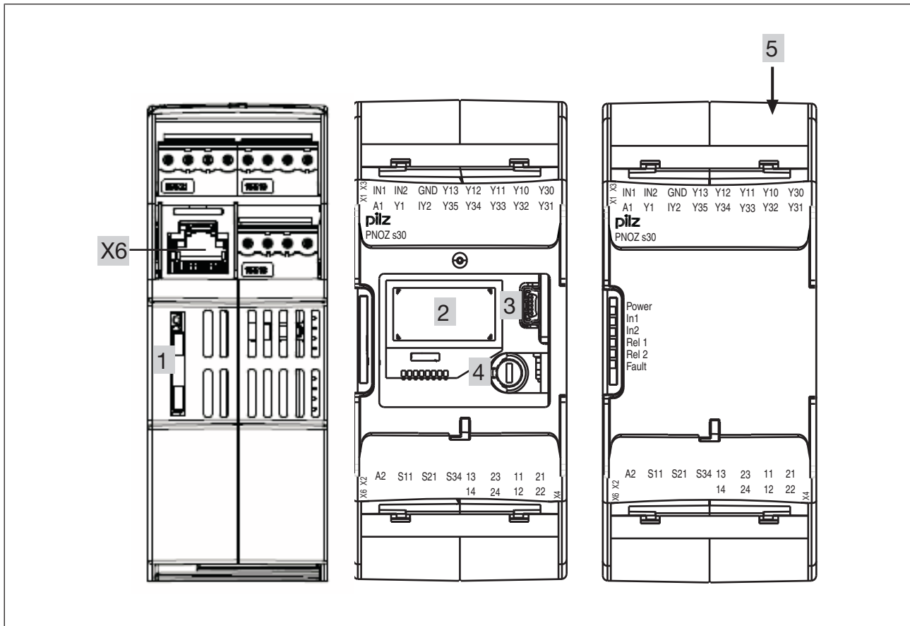
Fig.: Left: Side view, centre: Front view without cover, right: Front view with cover
